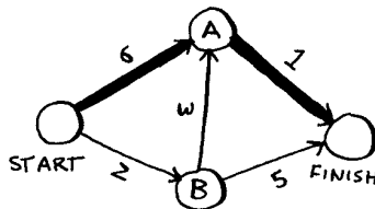
SHORTEST PATH WITH BREADTH-FIRST SEARCH
